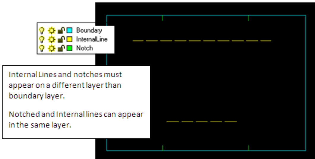
Figure 1: Notches and Internal lines in DXF files. Download DXF example
